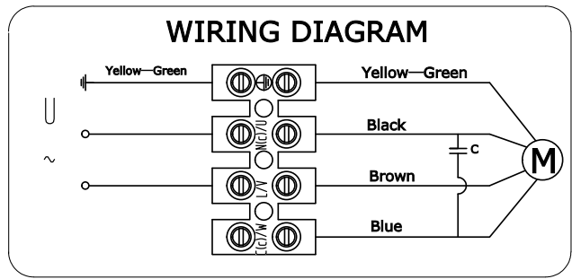
WIRING DIAGRAM (接线图):
