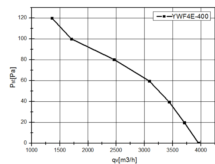
FLOW RATE CURVE (风量曲线):
